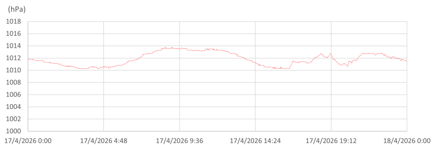
24-hour Time Series of Mean Sea Level Pressure
