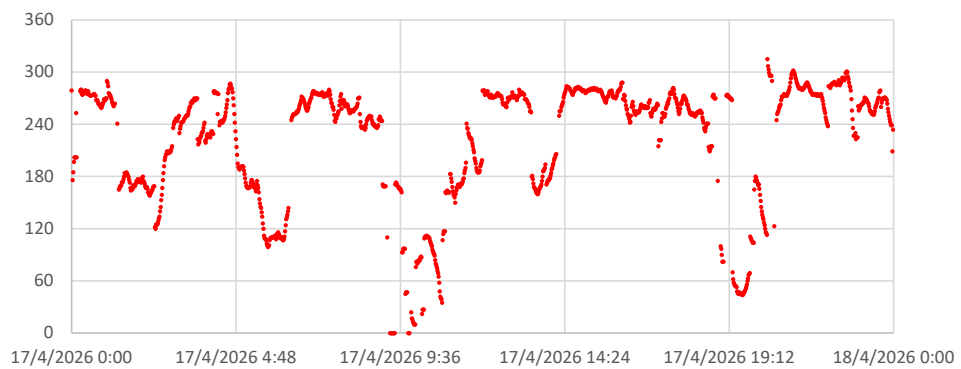
24-hour Time Series of 10-minute Mean Wind Direction
