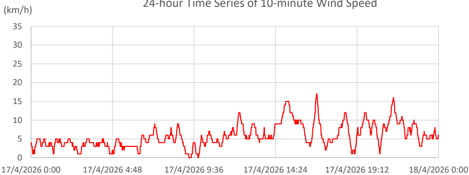
24-hour Time Series of 10-minute Wind Speed
