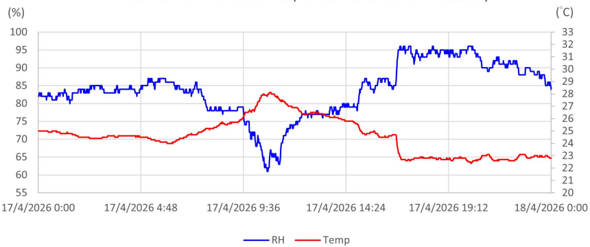
24-hour Time Series of Air Temperature and Relative Humidity
