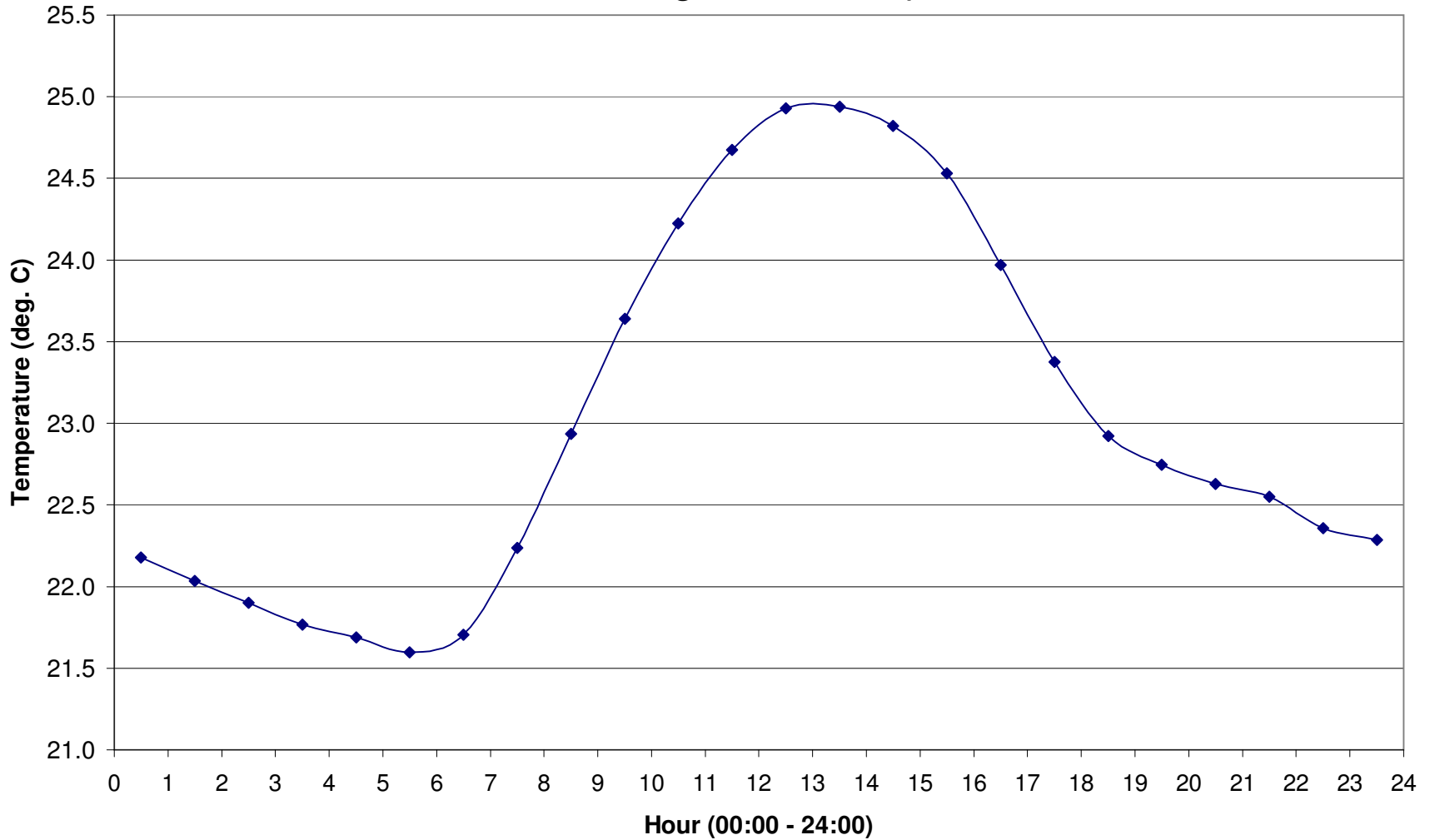
Annual average 24-hour Variation of Annual Average Temperature in 2010 (data from King's Park station)
