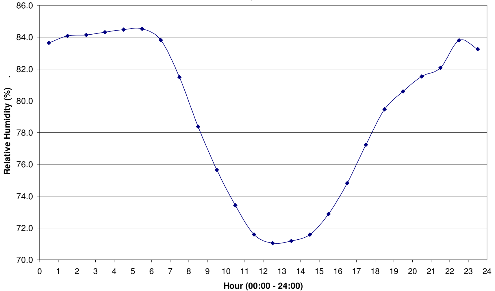
Annual average 24-hour Variation of Annual Average Relative Humidity in 2010 (data from King's Park station)
